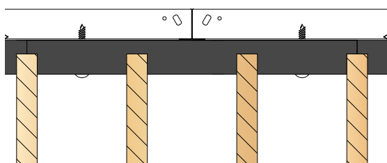
Baffle Series 1 (square)
